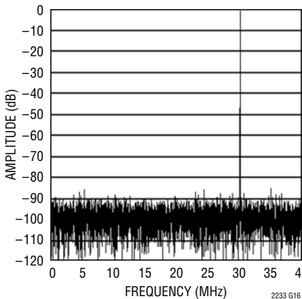
LTC2233: 8192 Point FFT, f_{IN} = 30\text{MHz} , -1\text{dB} , 2V Range
