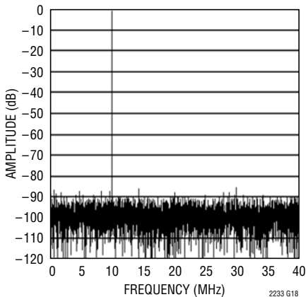
LTC2233: 8192 Point FFT, f_{IN} = 70\text{MHz} , -1\text{dB} , 2V Range
