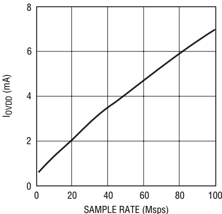
LTC2233: I_{VDD} vs Sample Rate, 5MHz Sine Wave Input, -1\text{dB} , 0V_{DD} = 1.8\text{V}
