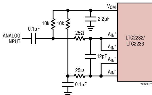
Figure 5. Single-Ended Drive
