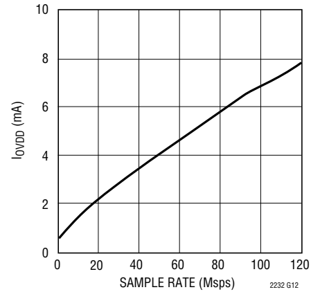
LTC2232: I_{OVD} vs Sample Rate, 5MHz Sine Wave Input, -1\text{dB} , 0V_{DD} = 1.8V
