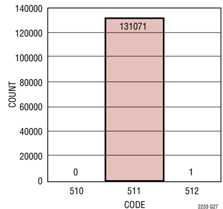
LTC2233: Noise Histogram
