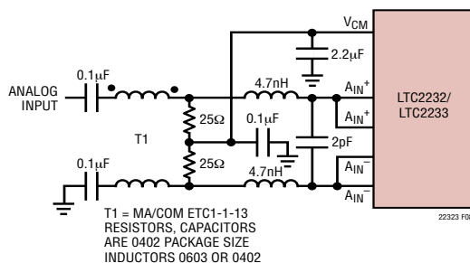
Figure 8. Recommended Front End Circuit for Input Frequencies Above 500MHz
