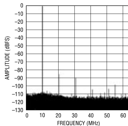
64K Point FFT, f_{IN} = 140.1 MHz, -1dB, PGA = 0
