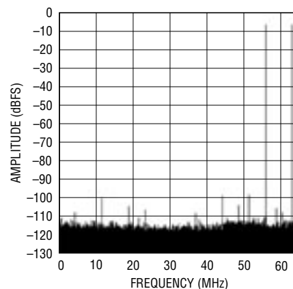
64K Point FFT, f_{IN1} = 67.2 MHz, -7dBFS, f_{IN2} = 74.4 MHz, -7dBFS, PGA = 0
