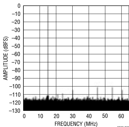
64k Point FFT, F_{IN} = 15.1\text{MHz} , -1dB, PGA = 0
