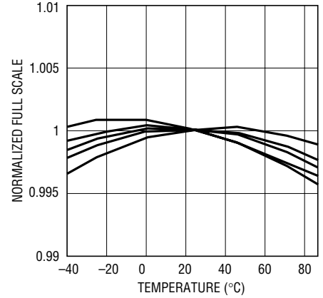
Normalized Full Scale vs Temperature, Internal Reference, 5 Units
