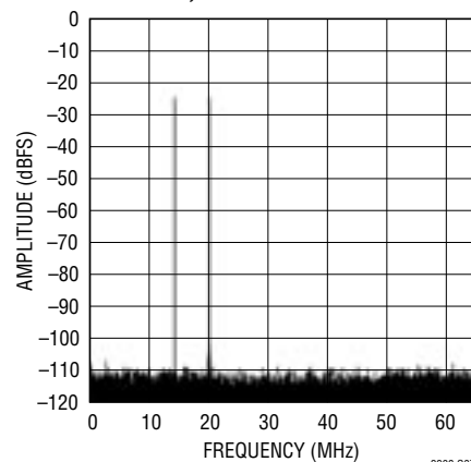
32k Point 2-Tone FFT, F_{IN} = 20.14\text{MHz} and 14.25\text{MHz} , -25dBFS, PGA = 0
