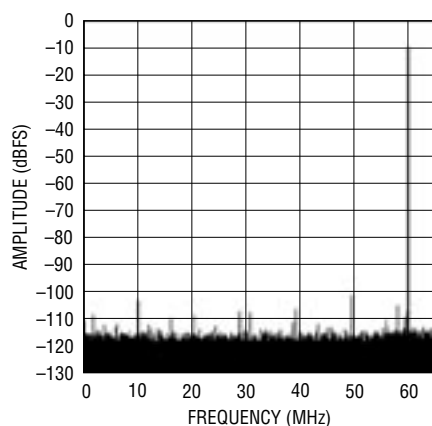
64K Point FFT, f_{IN} = 70.1 MHz, -10dB, PGA = 0
