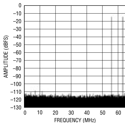
64K Point FFT, f_{IN1} = 67.2 MHz, -15dBFS, f_{IN2} = 74.4 MHz, -15dBFS, PGA = 0
