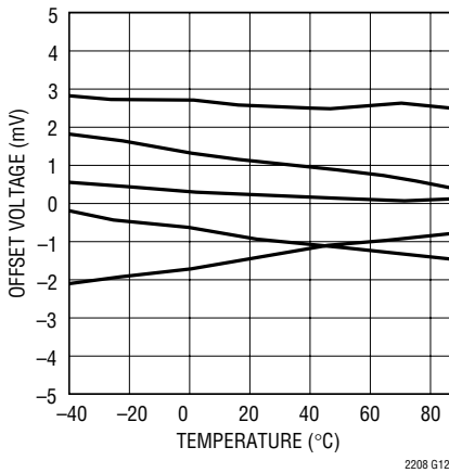
Input Offset Voltage vs Temperature, 5 Units
