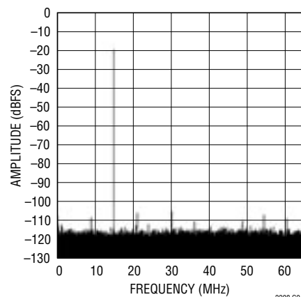
64k Point FFT, 15.1MHz, -20dBFS, PGA = 0, Internal Dither "Off"
