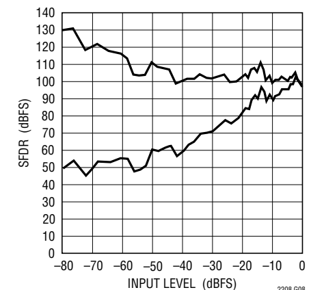
SFDR vs Input Level, F_{IN} = 15\text{MHz} , PGA = 0, Dither "Off"
