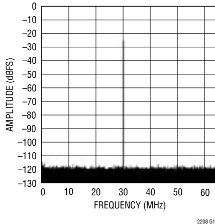
128K Point FFT, f_{IN} = 30.1\text{MHz} , -26dBFS, \text{PGA} = 0 , Dither "On"
