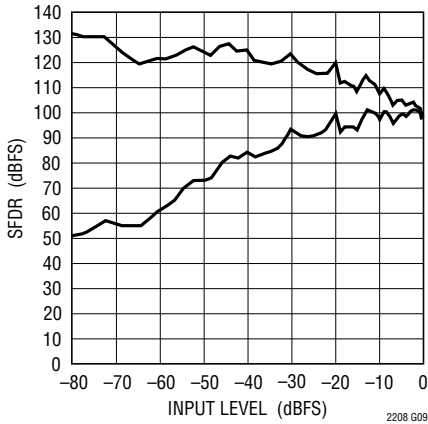
SFDR vs Input Level, f_{IN} = 15\text{MHz} , \text{PGA} = 0 , Dither "On"
