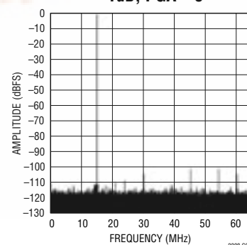
64k Point FFT, F_{IN} = 15.1\text{MHz} , -1dB, PGA = 0
