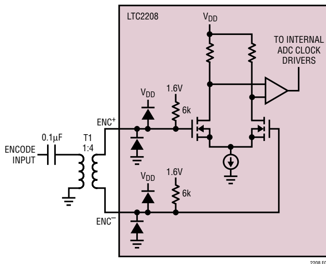
Figure 8. Transformer Driven Encode
