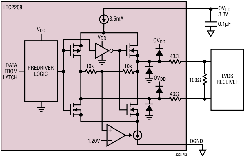
Figure 12. Equivalent Output Buffer in LVDS Mode Low Power LVDS
