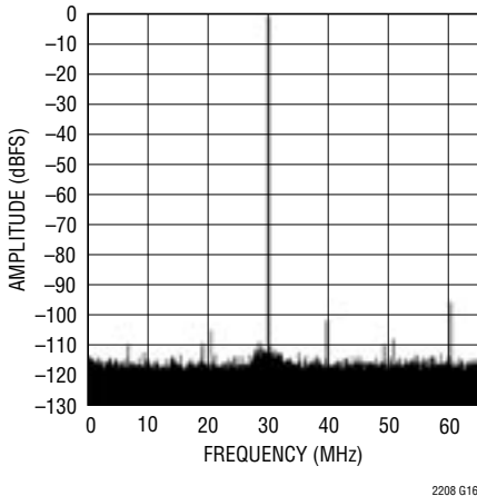
64K Point FFT, f_{IN} = 30\text{MHz} , -1dB, \text{PGA} = 0
