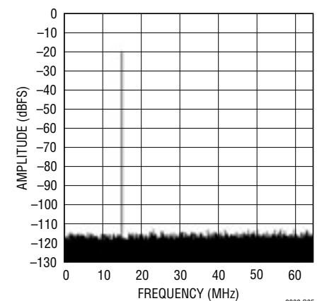
64k Point FFT, 15.1MHz, -20dBFS, PGA = 0, Internal Dither "On"
