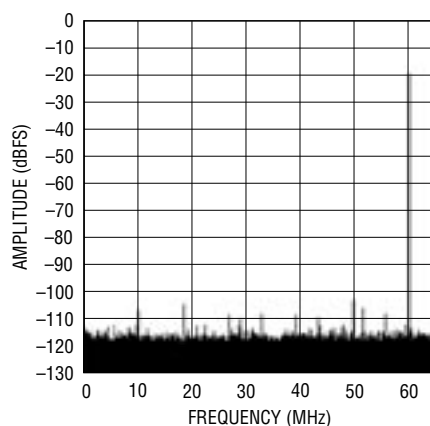
64K Point FFT, f_{IN} = 70.1 MHz, -20dB, PGA = 0
