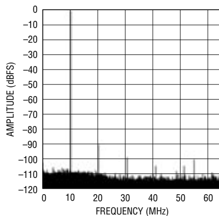
64K Point FFT, f_{IN} = 140.1 MHz, -1dB, PGA = 1
