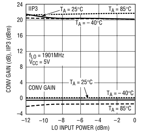
Conv Gain, IIP3 vs LO Input Power
