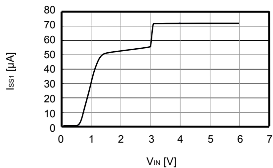
S-1170B30 ( T_a=25^\circ\text{C} )
