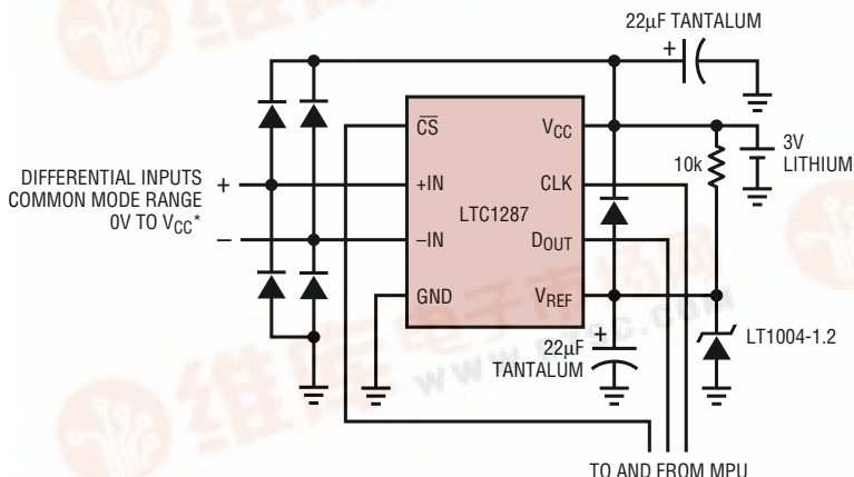
3V Differential Input Data Acquisition System
