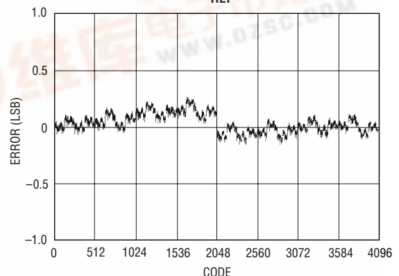
INL with V_{REF} = 1.2V
