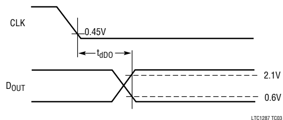
Voltage Waveforms for D_{OUT} Delay Time, t_{dD}
