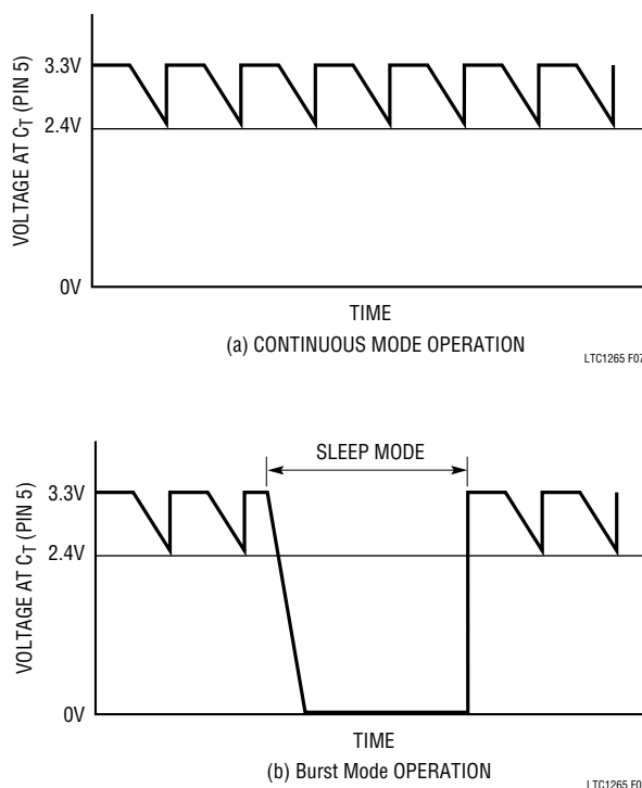
Figure 7. C_T Waveforms
