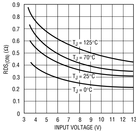
Switch Resistance
