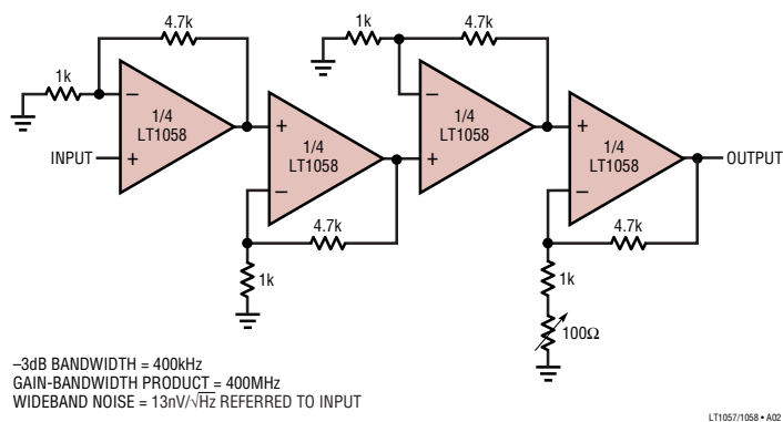
Wideband, High Input Impedance, Gain = 1000 Amplifier
