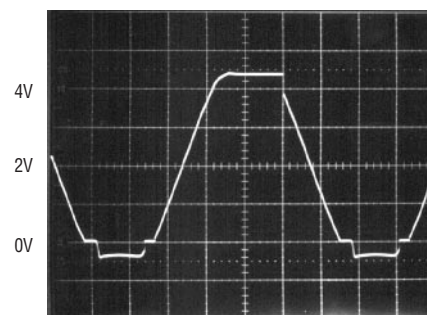
1ms/DIV LT2078/LT2079 NO PHASE REVERSAL
