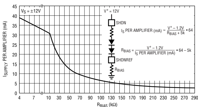
Figure 3. R_{\text{BIAS}} to Ground Current Control
