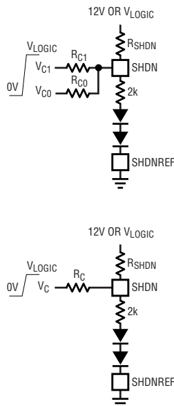
Figure 4. Providing Logic Input Control of Operating Current
