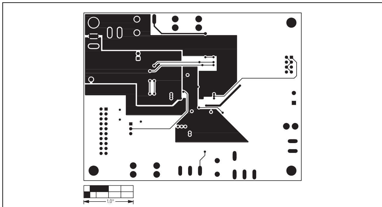
Figure 9. MAX9765 EV Kit PC Board Layout—Solder Side
