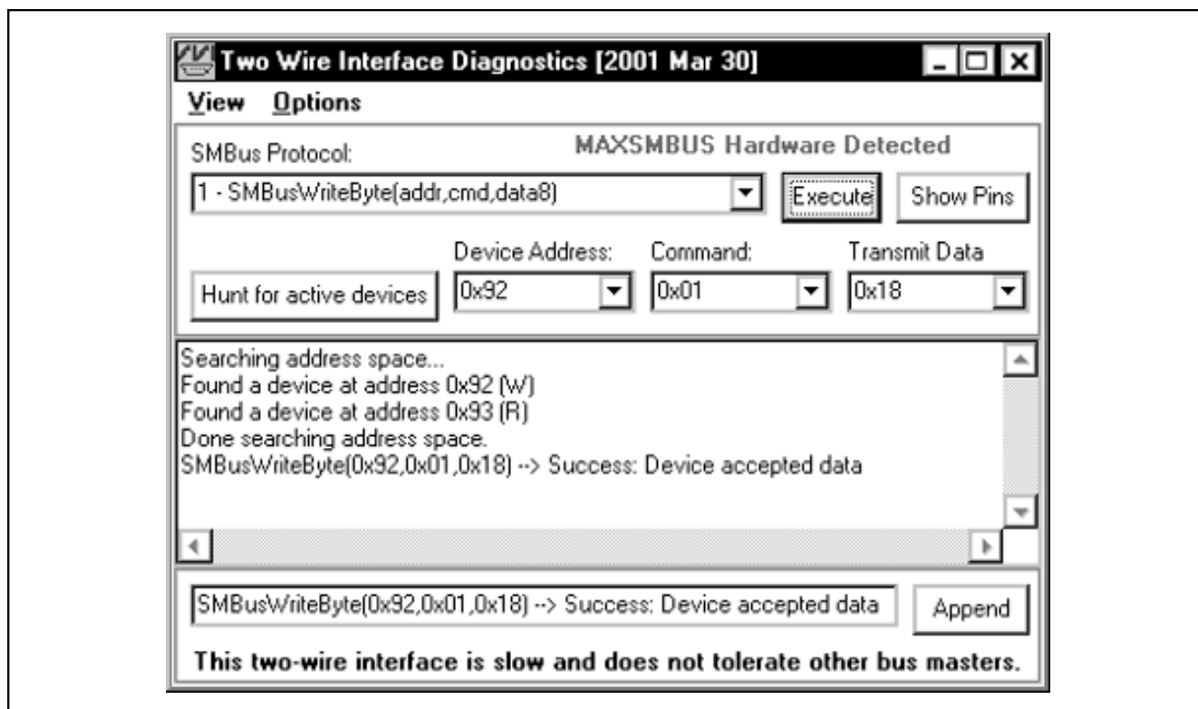
Figure 3. Simple SMBusWriteByte Operation Using the Included 2-Wire Interface Diagnostics. (In this example, the software is writing data (0x18) to Device Address 0x92, Register Address 0x01. The above data sequence mutes both MAX9765 output channels.)
