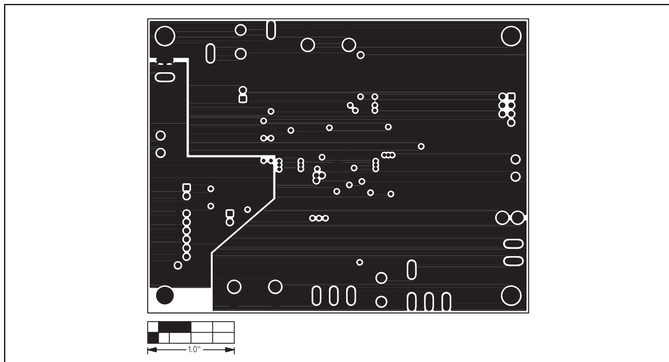
Figure 7. MAX9765 EV Kit PC Board Layout—Inner Layer 2
