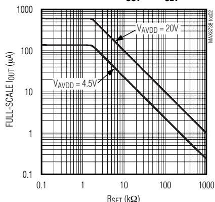
FULL-SCALE I OUT vs. R SET
