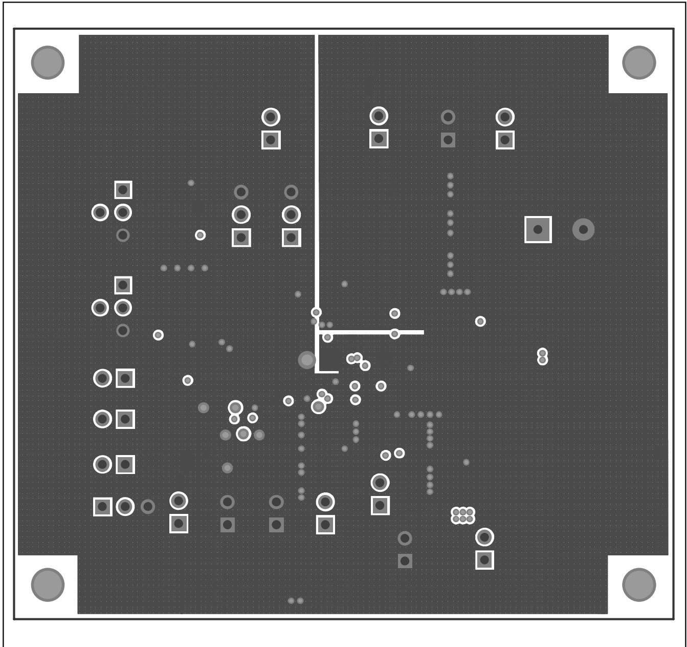
Figure 5. MAX8632 EV Kit PC Board Layout—Inner Layer 3
