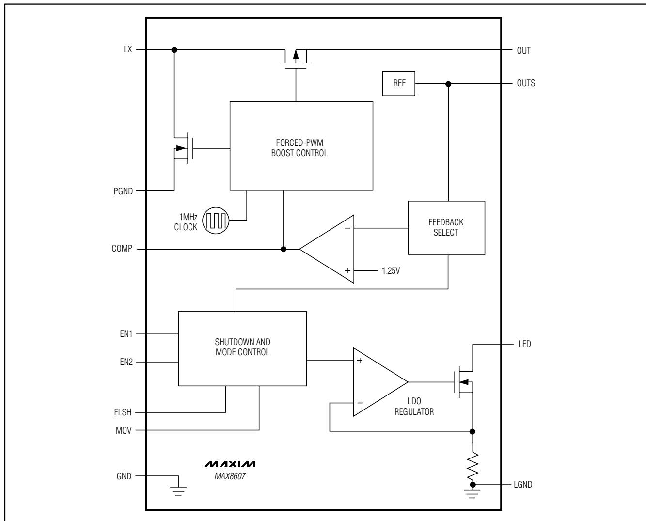
Figure 1. Functional Diagram
