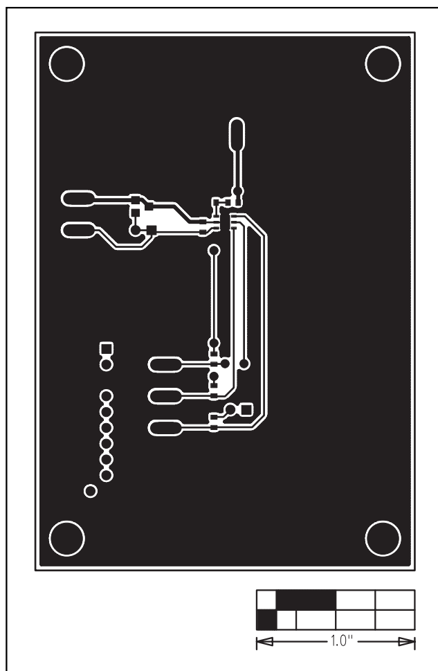
Figure 4. MAX6642 EV Kit PC Board Layout—Component Side
