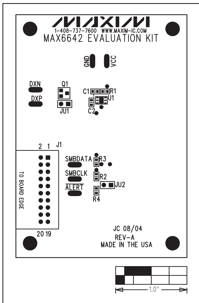
Figure 3. MAX6642 EV Kit Component Placement Guide—Component Side
