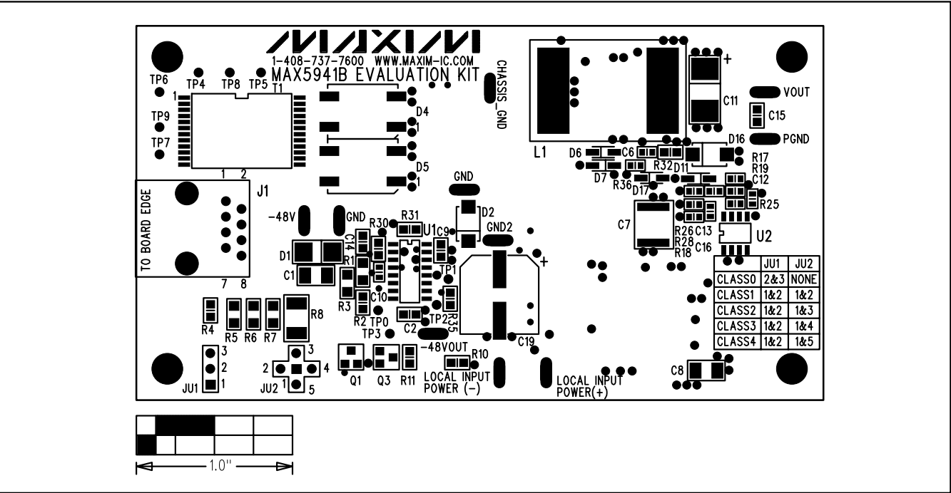
Figure 3. MAX5941B EV Kit Component Placement Guide—Component Side
