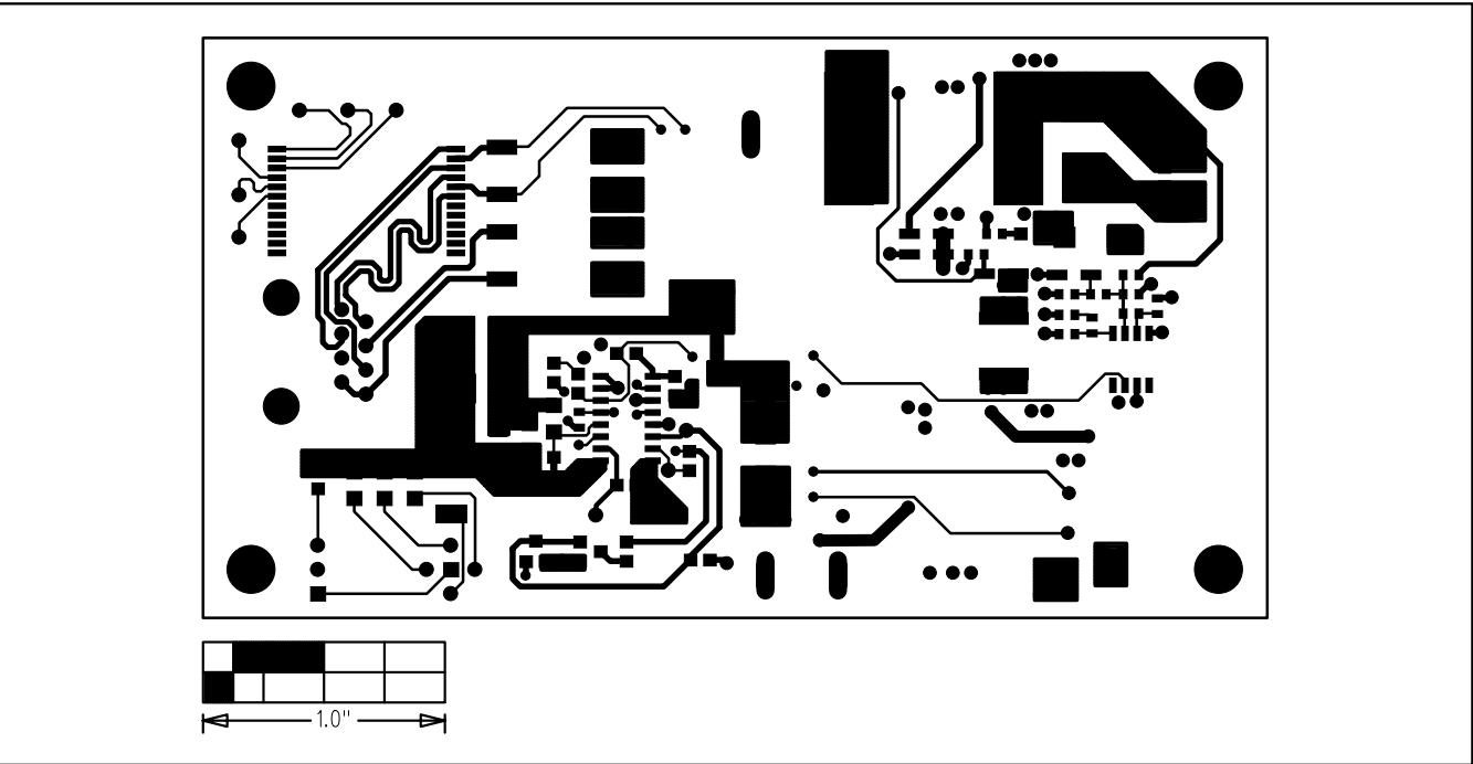
Figure 4. MAX5941B EV Kit PC Board Layout—Component Side
