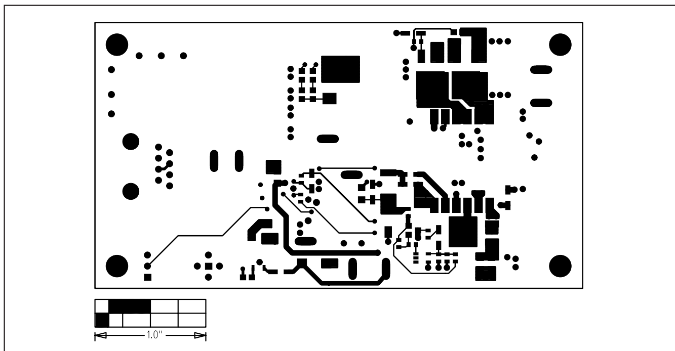
Figure 7. MAX5941B EV Kit PC Board Layout—Solder Side
