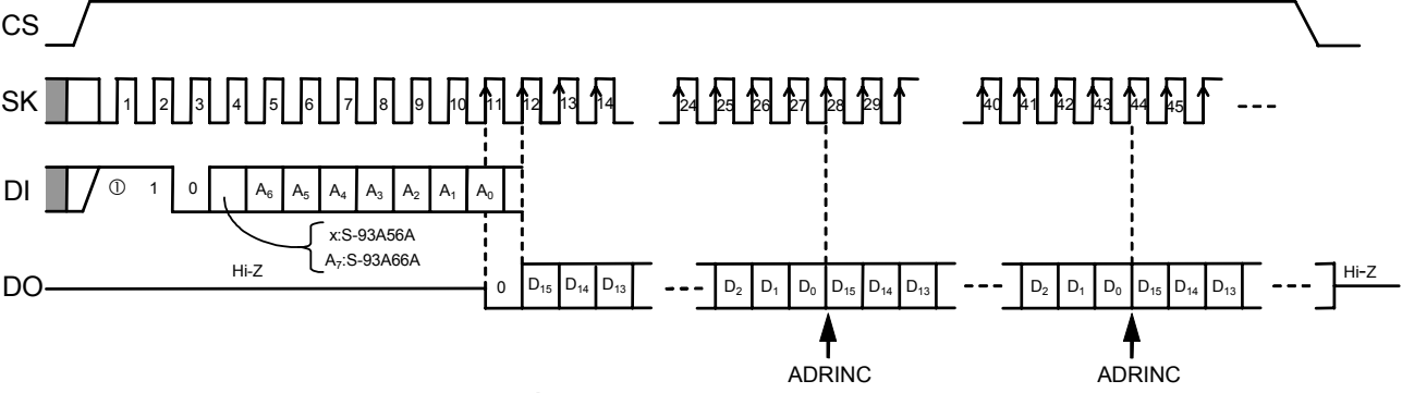
图5 读出定时 (S-93A56A, S-93A66A)
