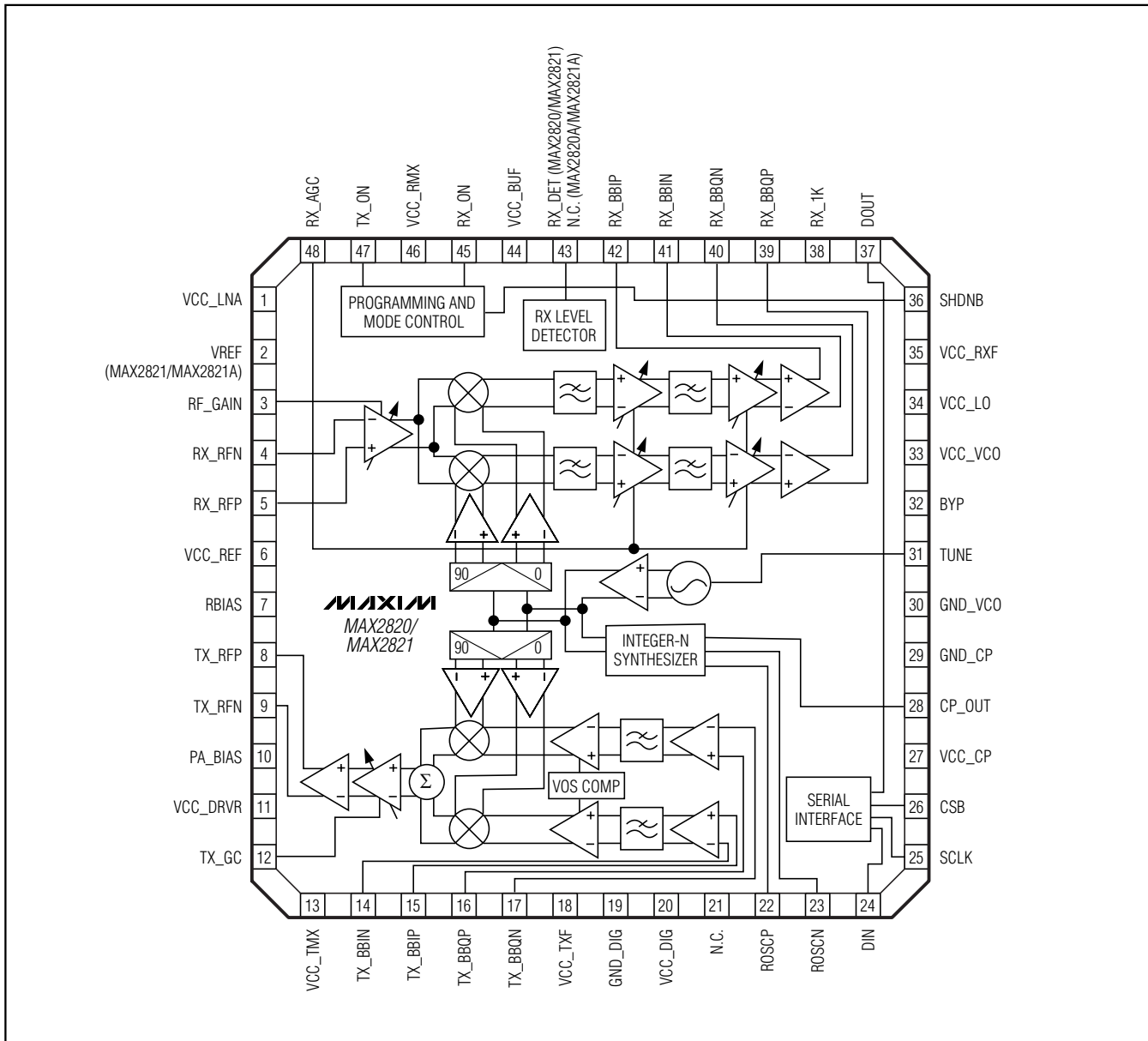
Pin Configuration/Functional Diagram
