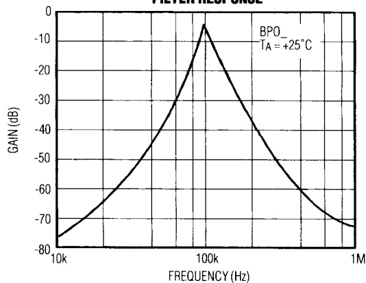
FILTER RESPONSE
