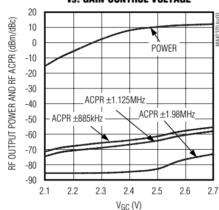
RF OUTPUT POWER AND RF ACPR vs. GAIN-CONTROL VOLTAGE
