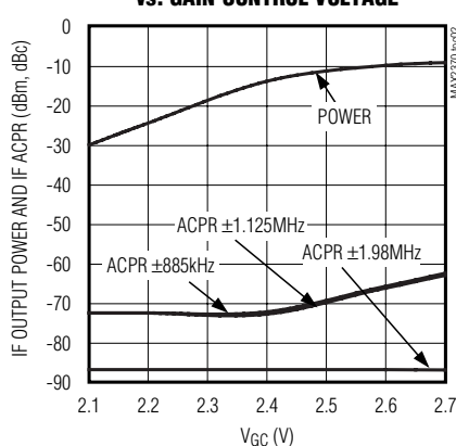
IF OUTPUT POWER AND IF ACPR vs. GAIN-CONTROL VOLTAGE
