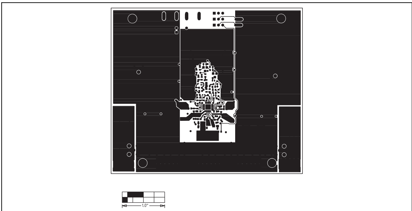
Figure 7. MAX1955 EV Kit PC Board Layout—Solder Side
