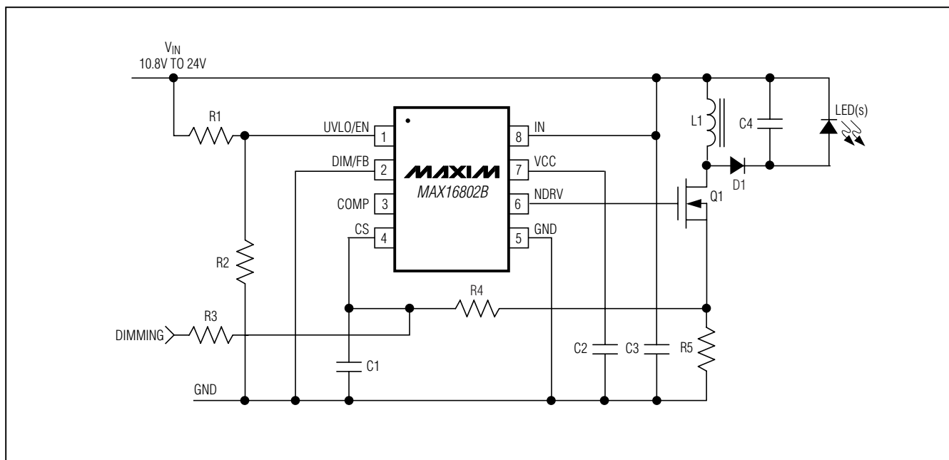
Figure 6. MAX16802 Flyback HB LED Driver with Dimming Capability, 10.8V to 24V Input Voltage Range
