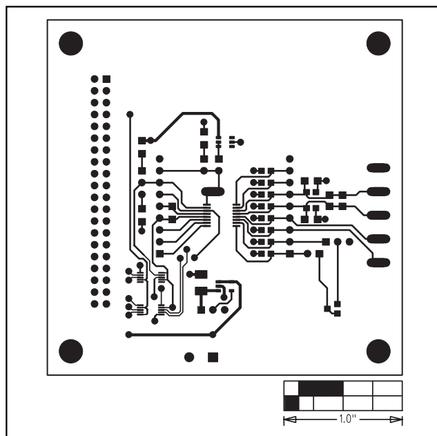
Figure 12. MAX1254 EV Kit PC Board Layout—Component Side
