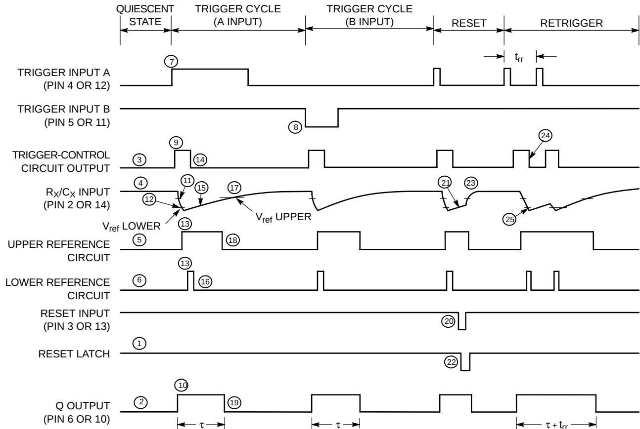
Figure 12. Timing Diagram
