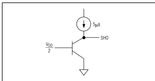
Figure 7. SHO Output Circuit
