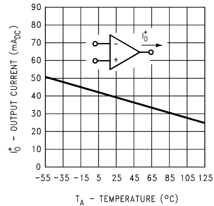
Current Limiting
