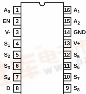
DG408/883 (CERDIP) TOP VIEW
