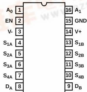
DG409/883 (CERDIP) TOP VIEW
