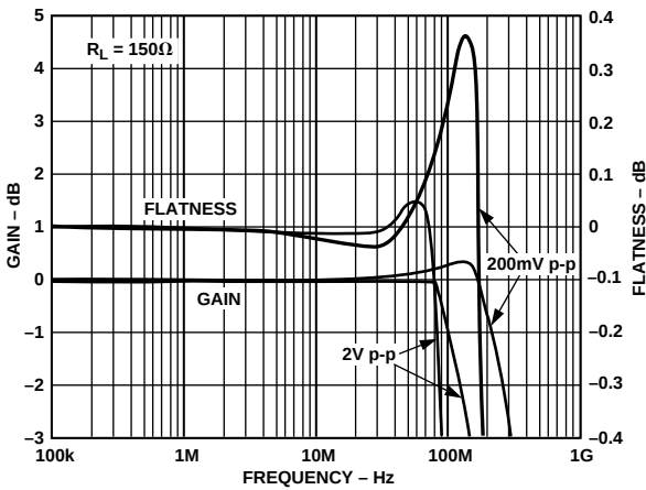
Figure 6. AD8108 Frequency Response
