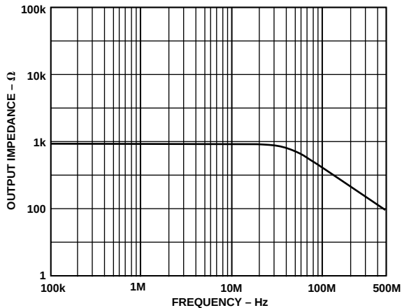
Figure 26. AD8109 Output Impedance, Disabled
