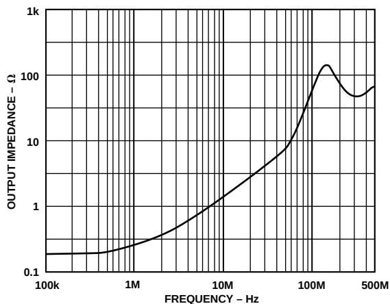
Figure 23. AD8108 Output Impedance, Enabled
