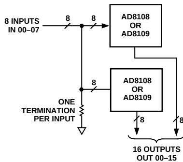
Figure 42. 8 × 16 Crosspoint Array Using Two AD8108s (Unity Gain) or Two AD8109s (Gain-of-Two)
