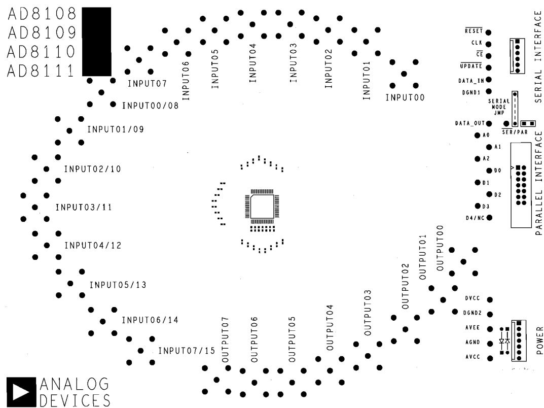
Figure 47. Component Side Silkscreen
