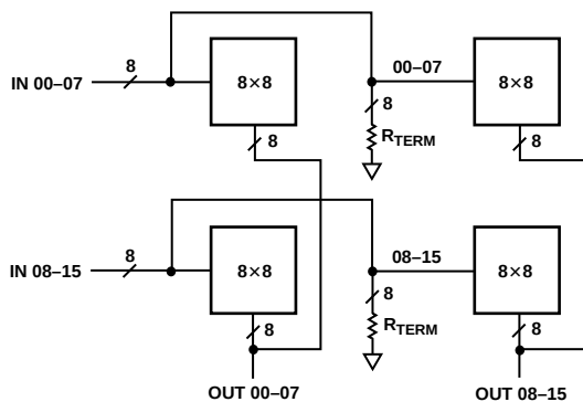
Figure 43. 16 × 16 Crosspoint Array Using Four AD8108s or AD8109s
