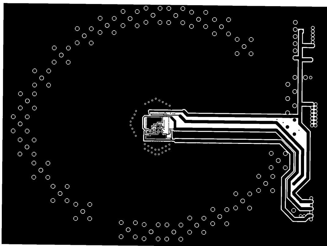
Figure 50. Board Layout (Power Plane)
