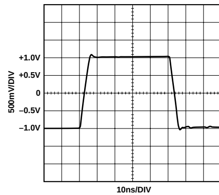
Figure 10. AD8108 Step Response, 2 V Step
