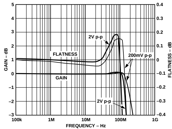
Figure 12. AD8109 Frequency Response
