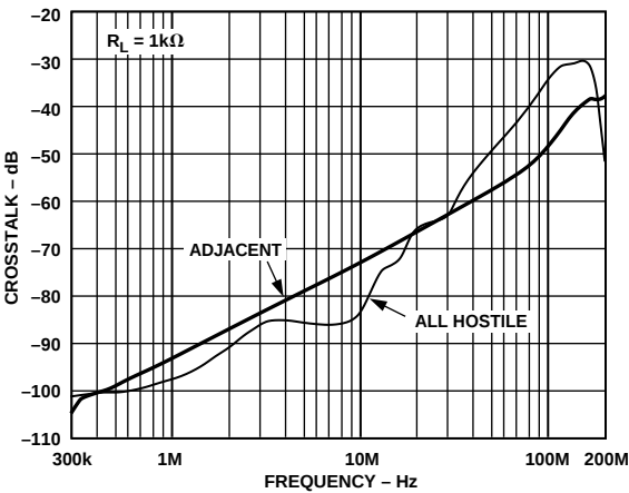
Figure 13. AD8109 Crosstalk vs. Frequency
