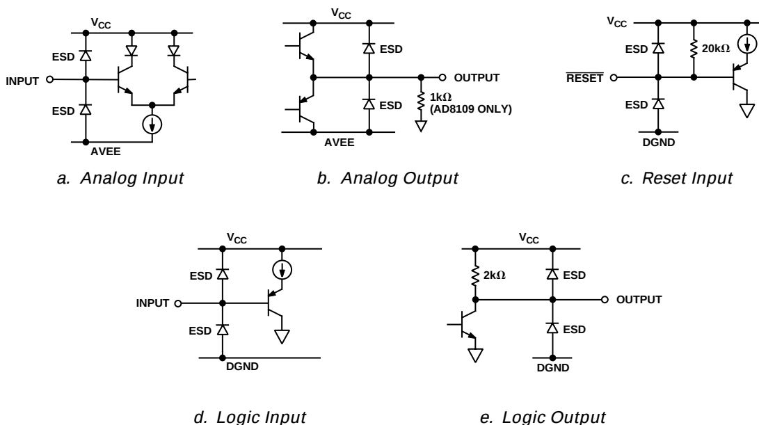
Figure 5. I/O Schematics
