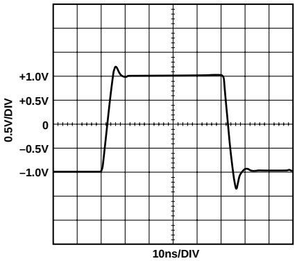
Figure 16. AD8109 Step Response, 2 V Step
