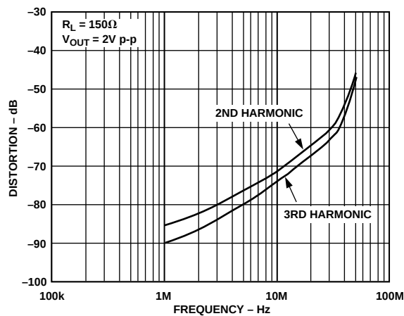
Figure 8. AD8108 Distortion vs. Frequency
