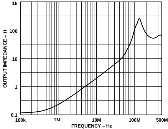
Figure 29. AD8109 Output Impedance, Enabled
