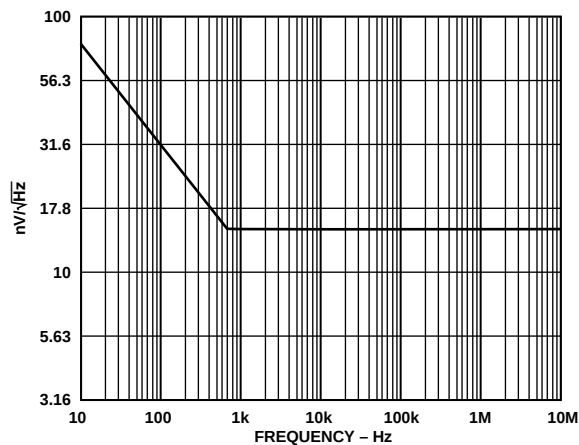
Figure 25. AD8109 Voltage Noise vs. Frequency
