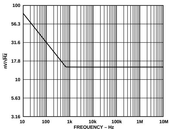
Figure 19. AD8108 Voltage Noise vs. Frequency
