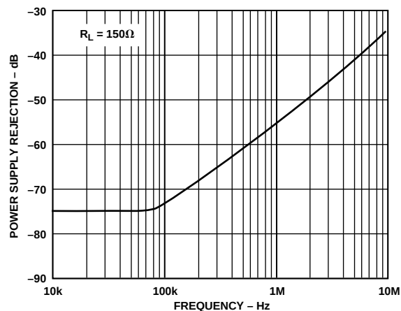
Figure 18. AD8108 PSRR vs. Frequency
