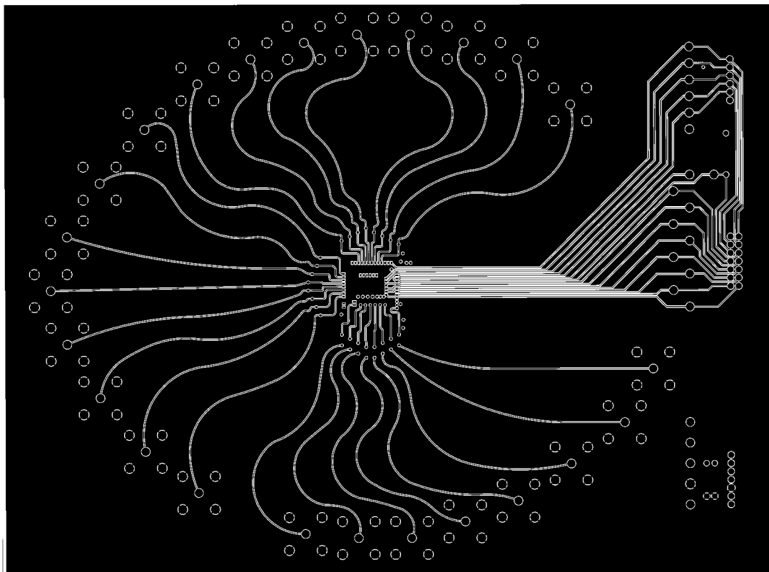
Figure 49. Board Layout (Signal Layer)
