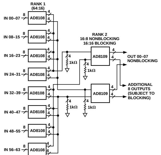
Figure 45. Nonblocking 64 × 8 Array with Gain-of-Two (64 × 16 Blocking)
