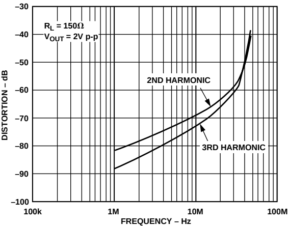
Figure 14. AD8109 Distortion vs. Frequency
