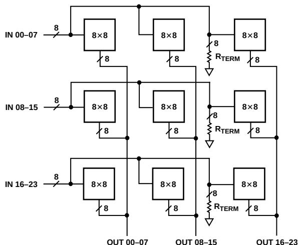
Figure 44. 24 × 24 Crosspoint Array Using Nine AD8108s or AD8109s
