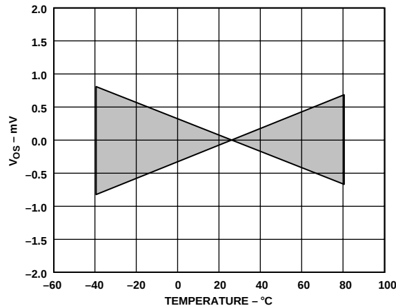
Figure 41. AD8109 Offset Voltage Drift vs. Temperature (Normalized at +25 ^{\circ}\text{C} )
