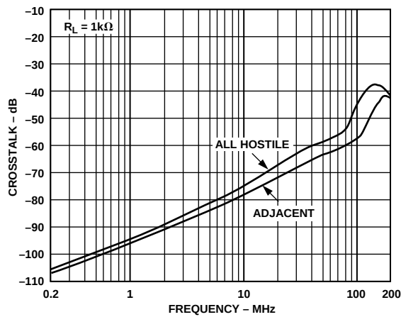
Figure 7. AD8108 Crosstalk vs. Frequency
