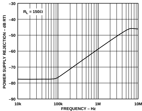
Figure 24. AD8109 PSRR vs. Frequency
