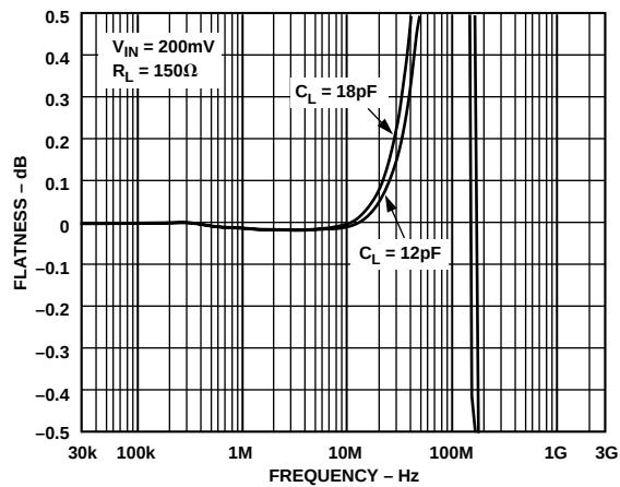
Figure 32. AD8108 Flatness vs. Capacitive Load
