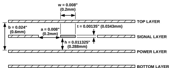
Figure 52. Cross Section of Input and Output Traces
