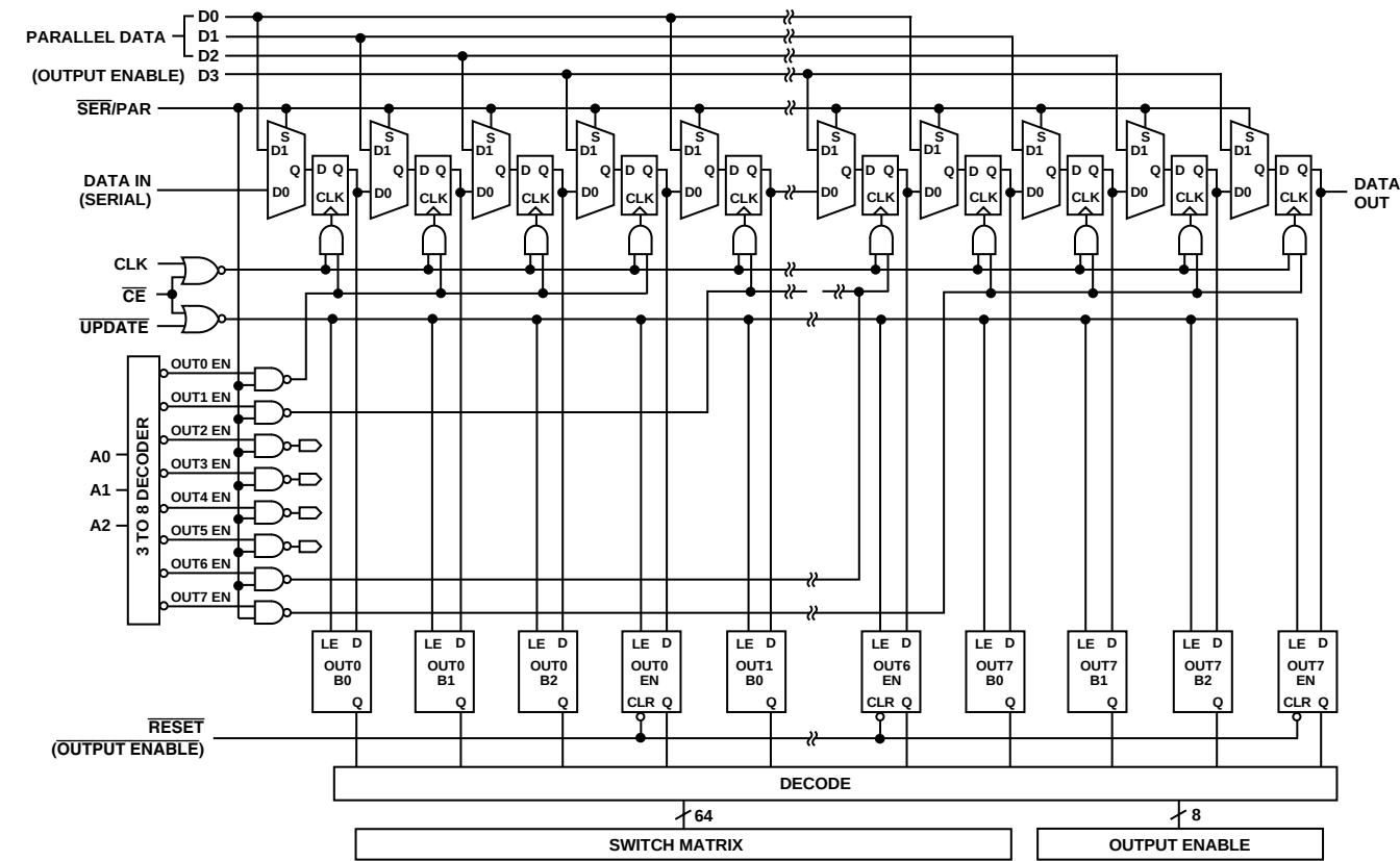
Figure 4. Logic Diagram
