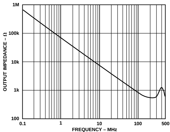
Figure 20. AD8108 Output Impedance, Disabled
