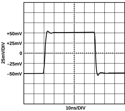
Figure 15. AD8109 Step Response, 100 mV Step
