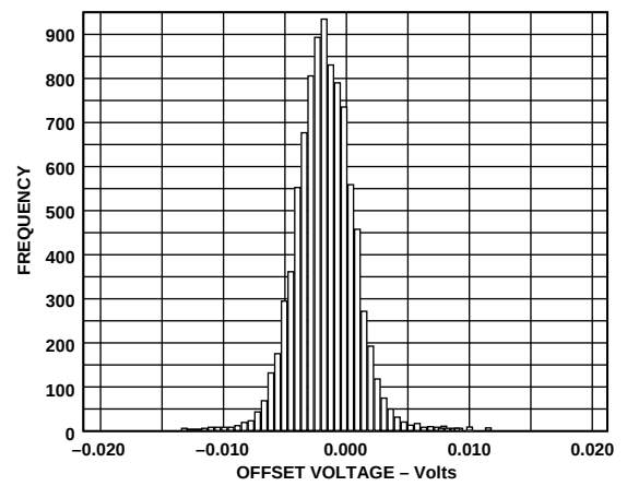
Figure 34. AD8108 Offset Voltage Distribution
