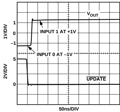
Figure 39. AD8109 Switching Time
