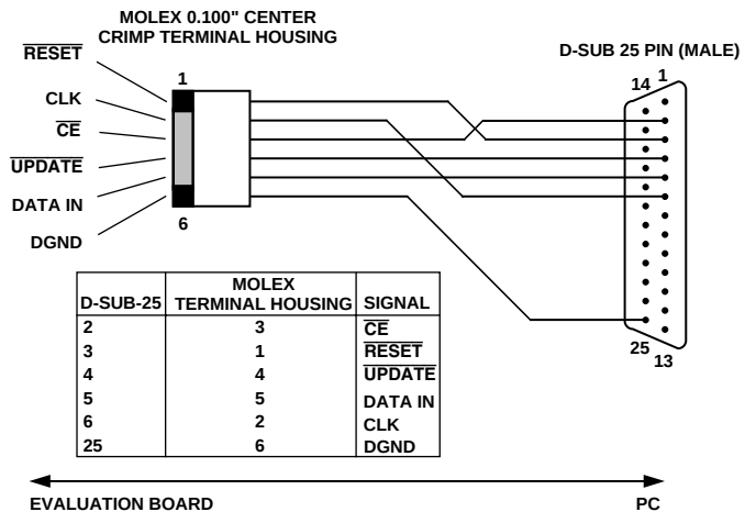
Figure 53. Evaluation Board-PC Connection Cable
