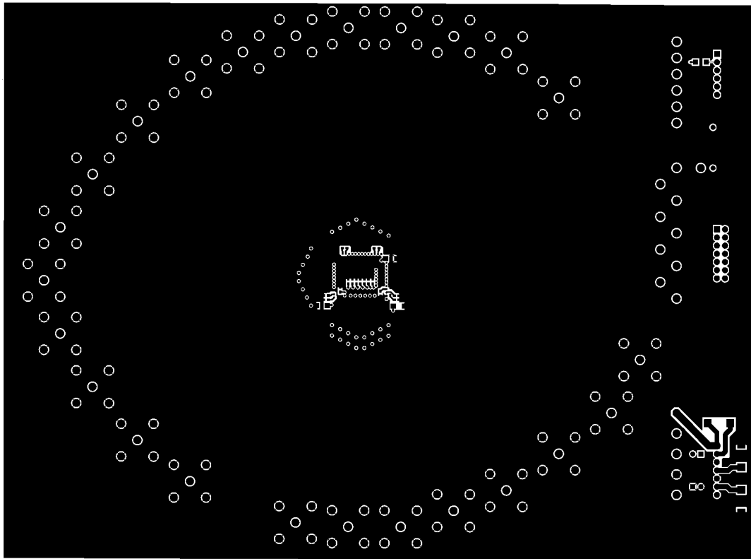
Figure 51. Board Layout (Bottom Layer)
