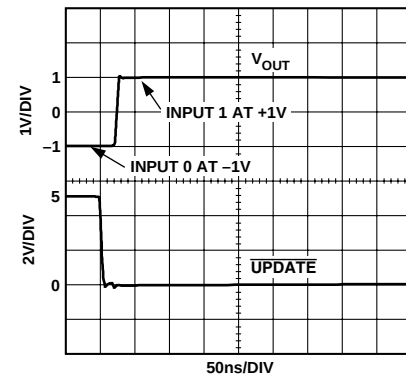
Figure 33. AD8108 Switching Time
