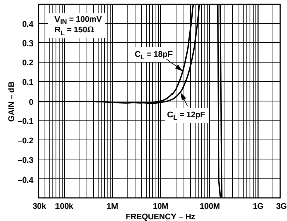
Figure 38. AD8109 Flatness vs. Capacitive Load
