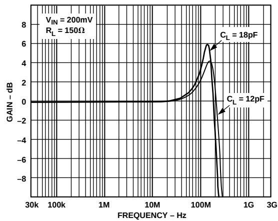
Figure 31. AD8108 Frequency Response vs. Capacitive Load
