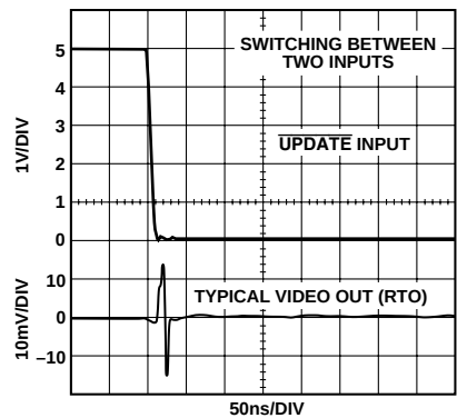
Figure 27. AD8109 Switching Transient (Glitch)
