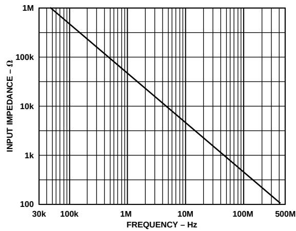
Figure 30. AD8108 Input Impedance vs. Frequency
