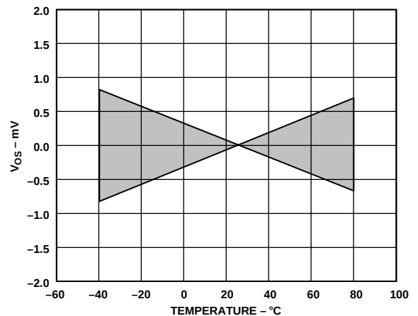
Figure 35. AD8108 Offset Voltage Drift vs. Temperature (Normalized at +25^{\circ}\text{C} )
