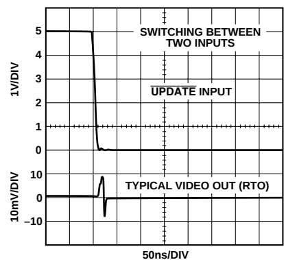
Figure 21. AD8108 Switching Transient (Glitch)
