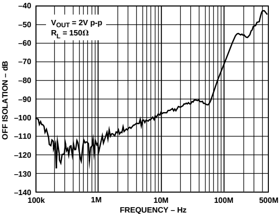
Figure 28. AD8109 Off Isolation, Input-Output
