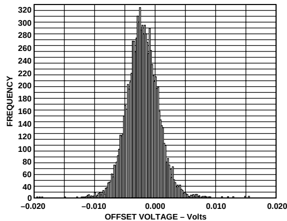
Figure 40. AD8109 Offset Voltage Distribution (RTI)
