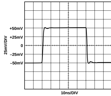
Figure 9. AD8108 Step Response, 100 mV Step
