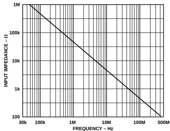
Figure 36. AD8109 Input Impedance vs. Frequency
