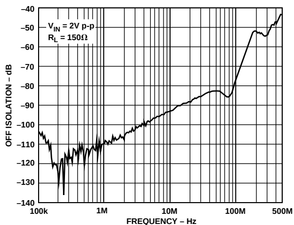
Figure 22. AD8108 Off Isolation, Input-Output
