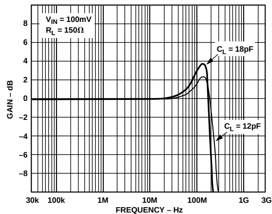
Figure 37. AD8109 Frequency Response vs. Capacitive Load
