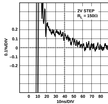
Figure 11. AD8108 Settling Time
