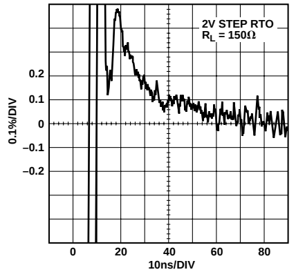
Figure 17. AD8109 Settling Time
