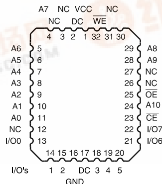
PLCC Top View
