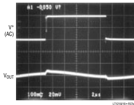
Figure 7b. LT1219 Power Supply Rejection Test
