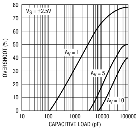
LT1218 Capacitive Load Handling
