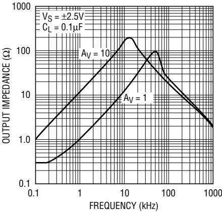
LT1219 Closed Loop Output Impedance vs Frequency
