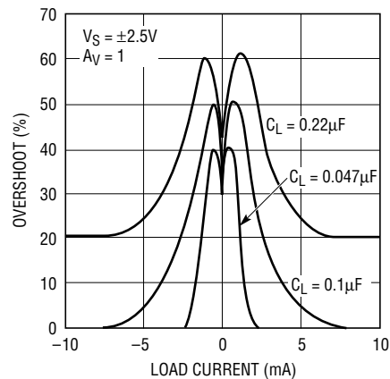
LT1219 Overshoot vs Load Current, V_S = \pm 2.5V
