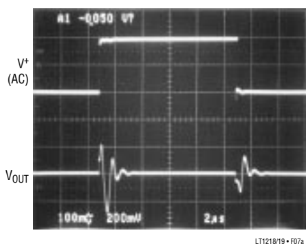
Figure 7a. LT1218 Power Supply Rejection Test
