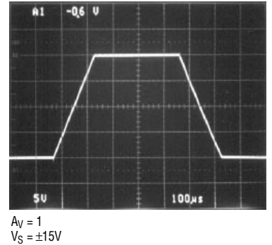
Large-Signal Response V_S = \pm 15\text{ V}
