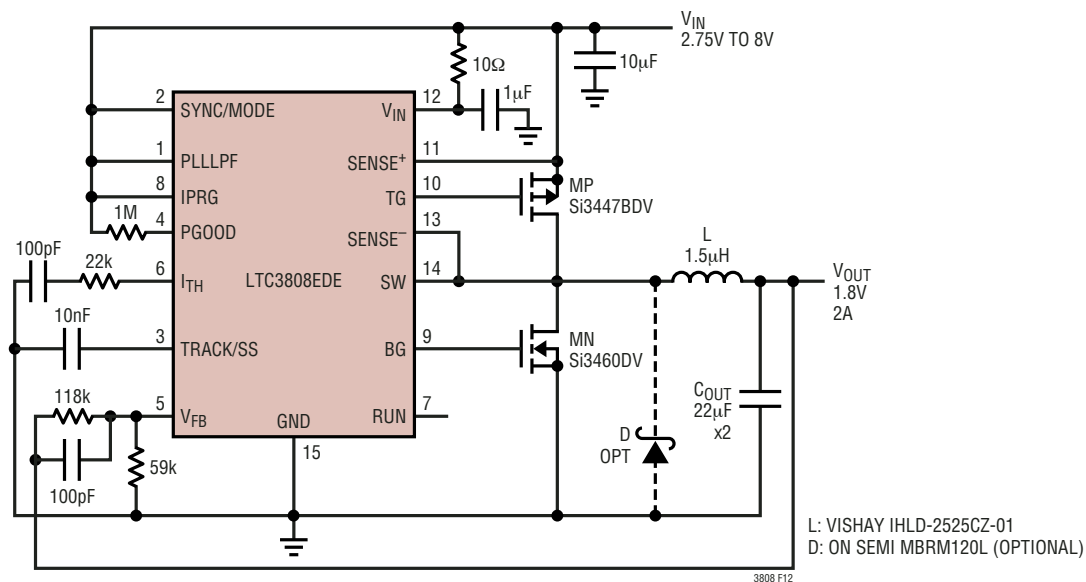
Figure 12. 750kHz, Synchronous DC/DC Converter with External Soft-Start, Ceramic Output Capacitor
