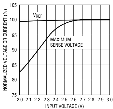
Figure 10. Line Regulation of V_{REF} and Maximum Sense Voltage
