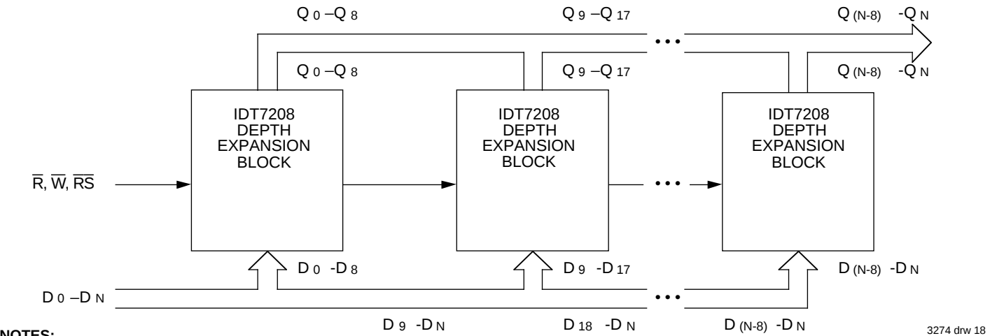
Figure 15. Compound FIFO Expansion
