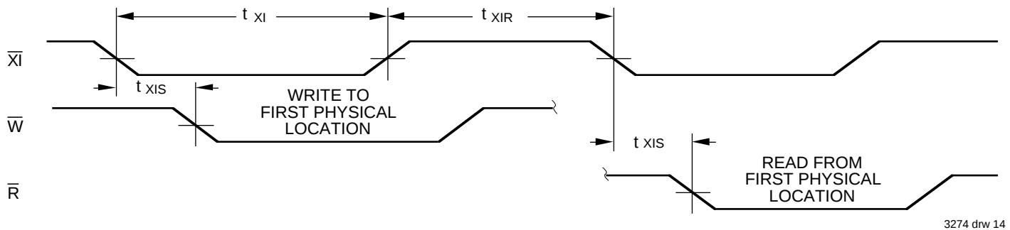
Figure 11. Expansion In
