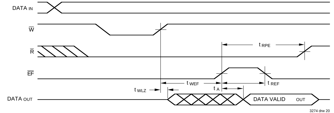
Figure 17. Read Data Flow-Through Mode
