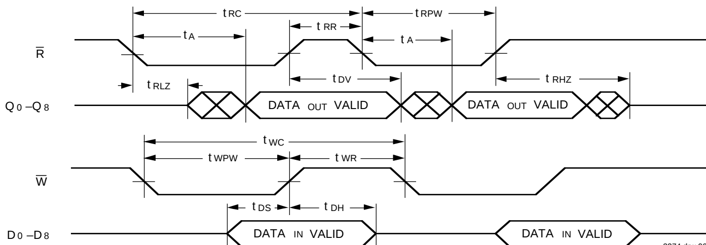
Figure 3. Asynchronous Write and Read Operation
