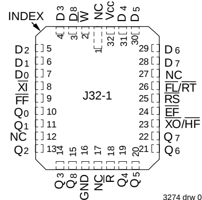
PLCC TOP VIEW
