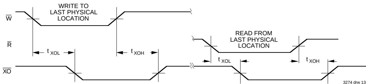
Figure 10. Expansion Out
