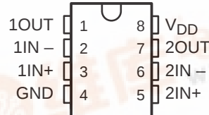
TLC1078 D, JG, OR P PACKAGE (TOP VIEW)
