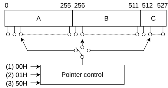
Figure 19. Pointer control
