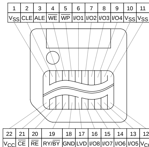
Figure 1. Pinout
