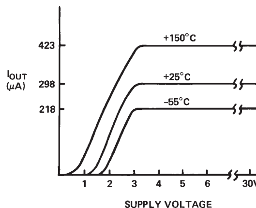
Figure 2. V-I Plot
