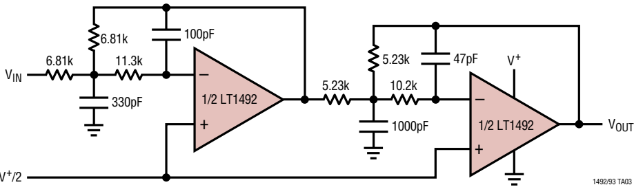
Single Supply 100kHz 4th Order Butterworth Filter
