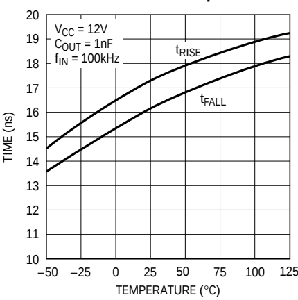
Rise/Fall Time vs Temperature
