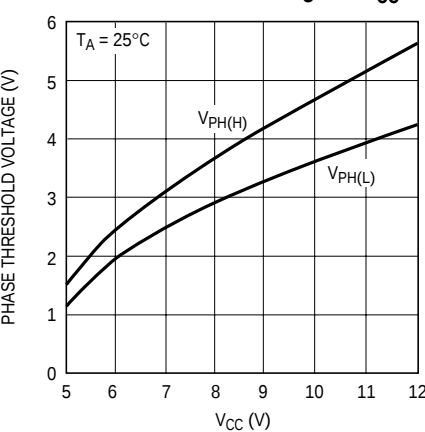
PHASE Threshold Voltage vs V_{CC}
