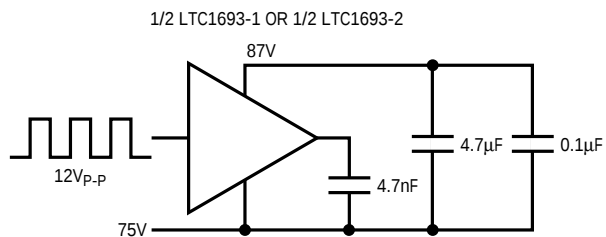
1/2 LTC1693-1 OR 1/2 LTC1693-2
