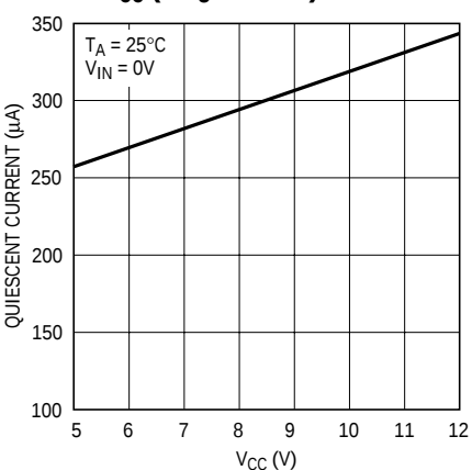
Quiescent Current vs V_{CC} (Single Driver)
