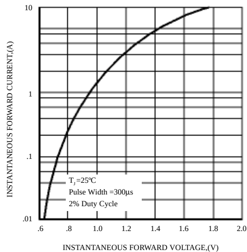
FIG.3-TYPICAL FORWARD CHARACTERISTICS
