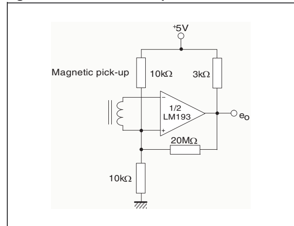
Figure 11. Transducer amplifier
