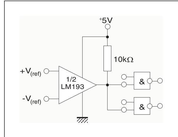
Figure 9. Driving CMOS
