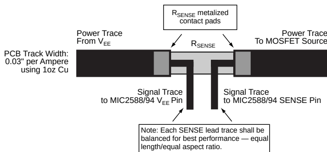
Figure 6. 4-Wire Kelvin Sense Connections for R_{SENSE}
