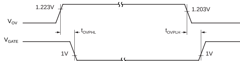
Figure 3. Overvoltage Response
