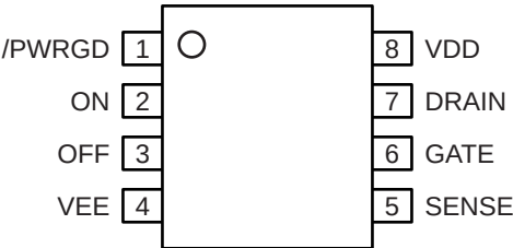
8-Pin SOIC (M) MIC2594-2BM
