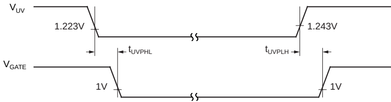
Figure 4. Undervoltage Response
