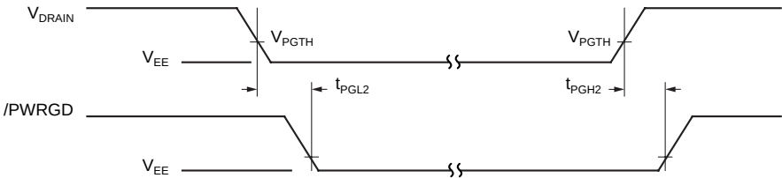
Figure 5. DRAIN to Power-Good Response
