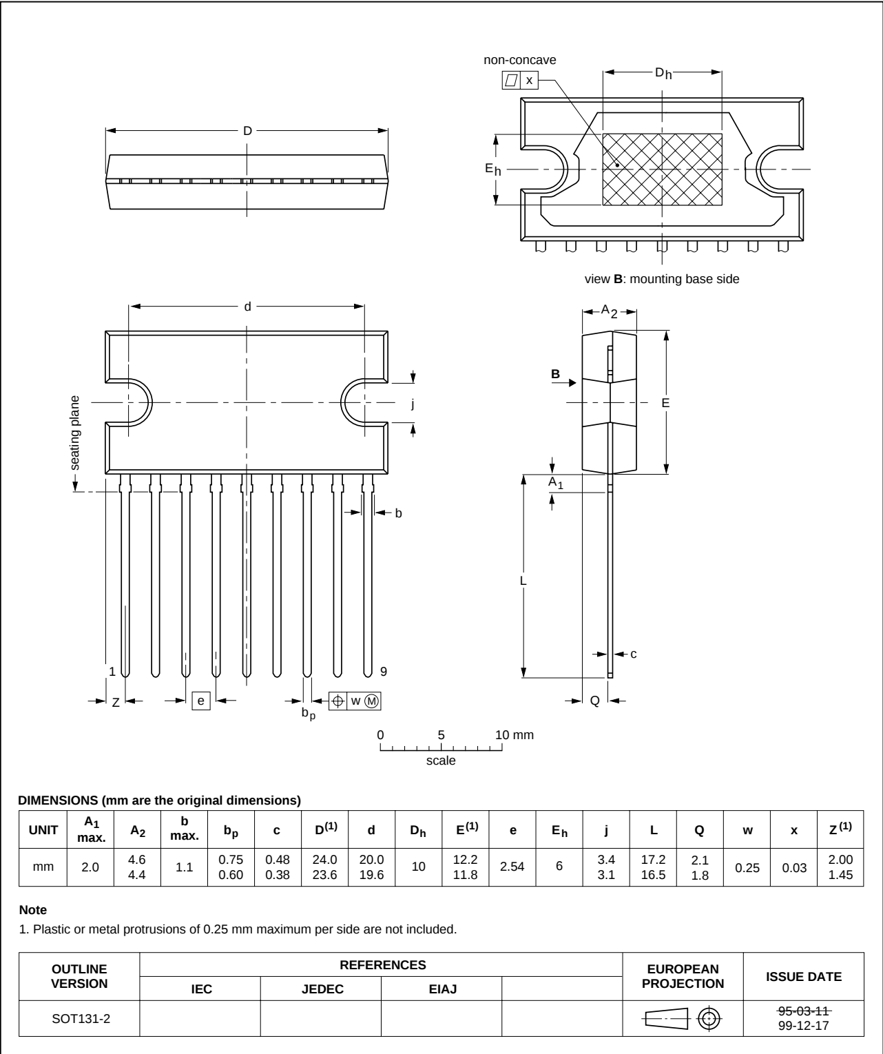
Fig 15. SIL9P package outline.
