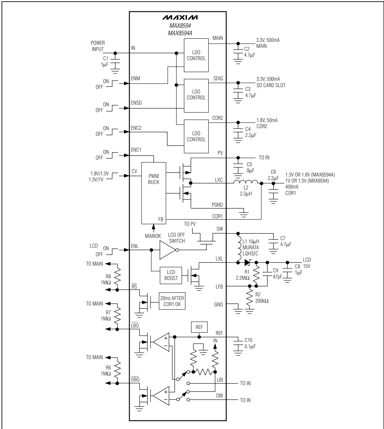
Figure 2. Block Diagram
