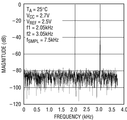
Intermodulation Distortion
