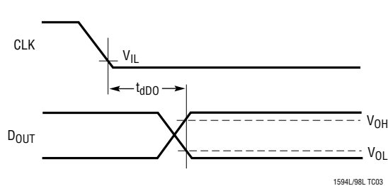
Voltage Waveforms for D OUT Delay Times, t dDO
