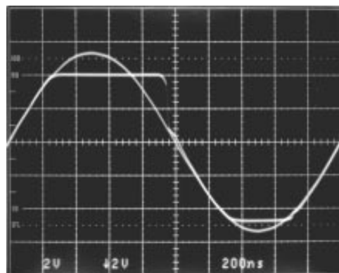
Overload Recovery
