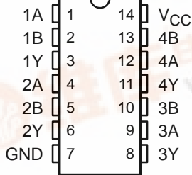
SN54AHCT32 ... J OR W PACKAGE SN74AHCT32 ... D, DB, DGV, N, NS, OR PW PACKAGE (TOP VIEW)
