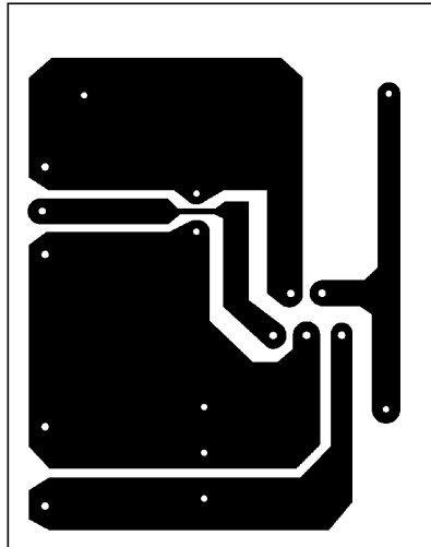
Copper Side
