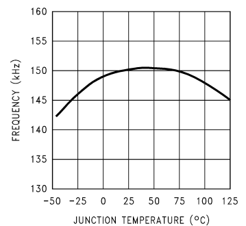
Switching Frequency
