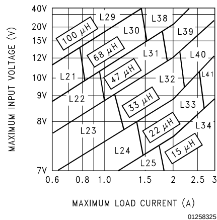
FIGURE 5. LM2596-5.0
