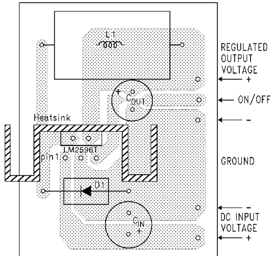
Component Side
