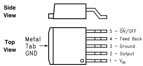
Surface Mount Package 5-Lead TO-263 (S)
