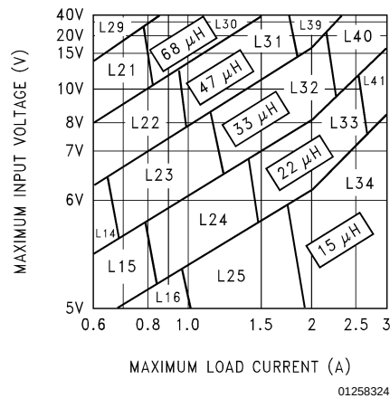
FIGURE 4. LM2596-3.3
