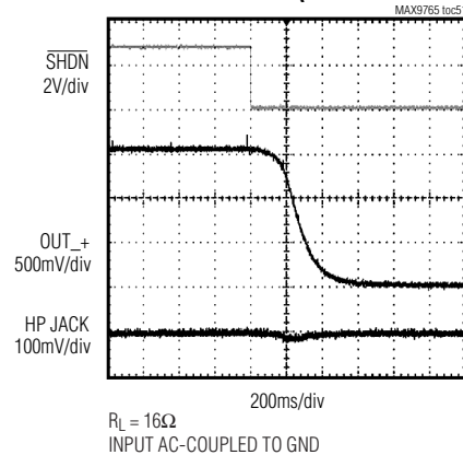
ENTERING SHUTDOWN (HEADPHONE MODE)
