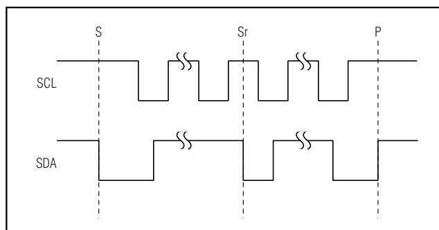
Figure 4. START/STOP Conditions
