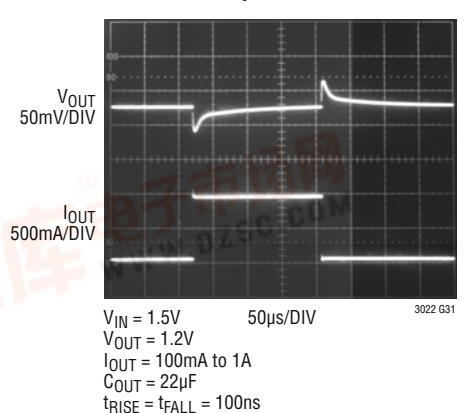
Transient Response
