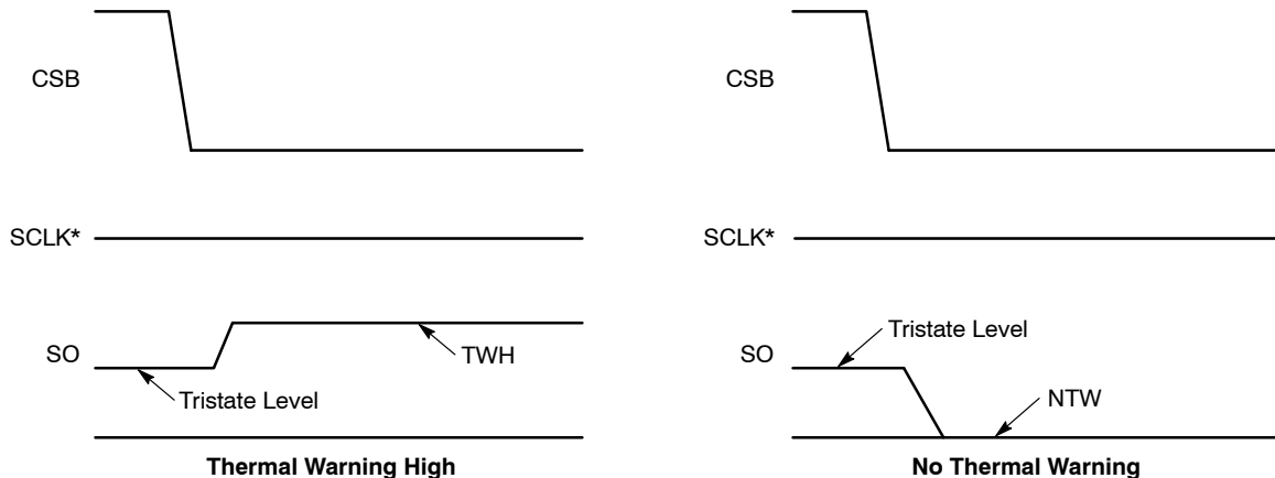
Figure 12. Access to Temperature Warning Information
