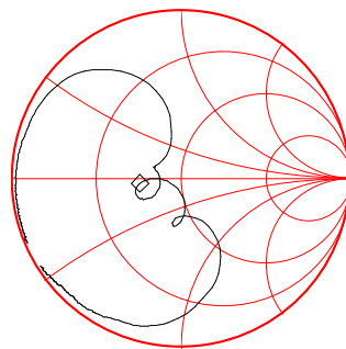
S11 Smith Chart
