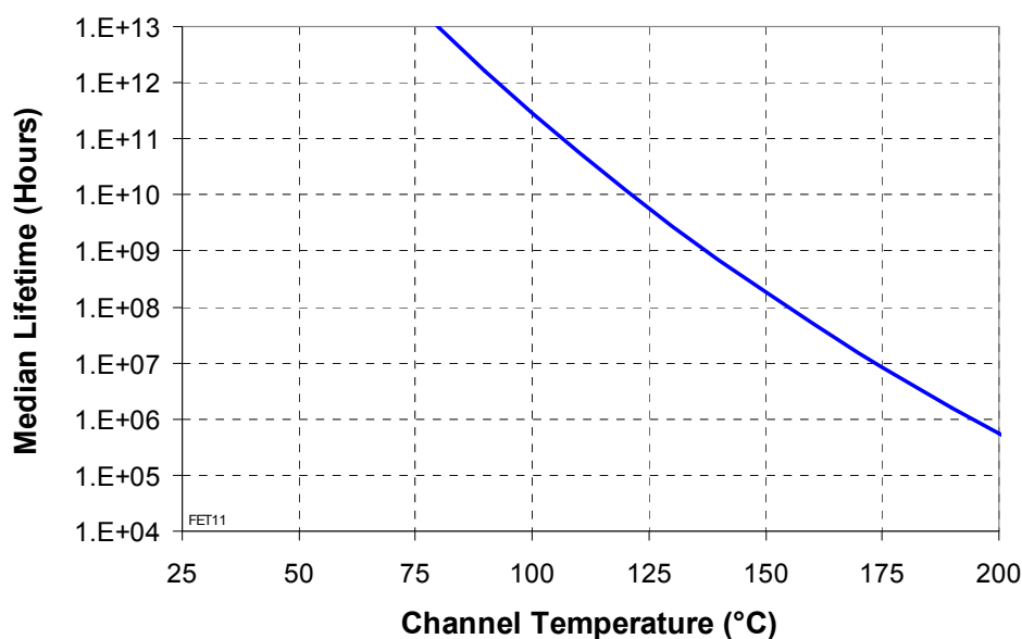
Median Lifetime (Tm) vs Channel Temperature
